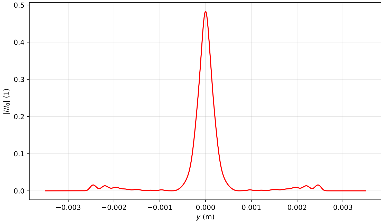
Intensity profile I(x=0, y, z=1.751)/I_0 , P_{in}=6.0P_{cr} , artificial time
